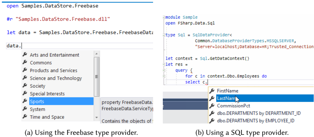
Fig. 5. Two examples of integrating information sources into F# using type providers, with strong typing and autocomplete.
